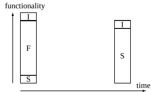
Figure 1: WOZ approach
